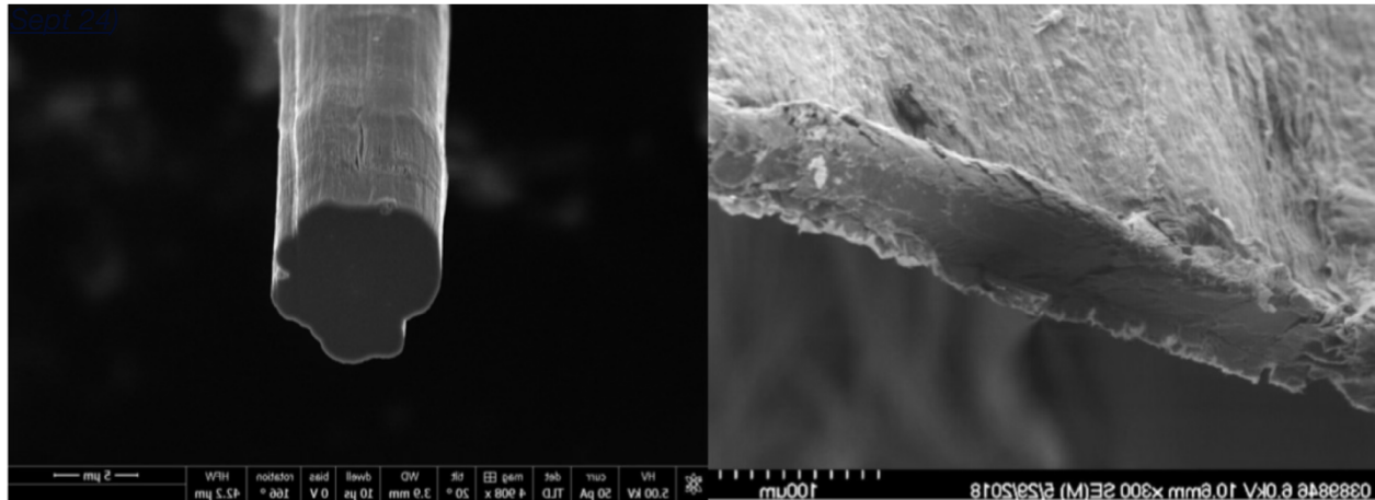
Carbon Nanotube
